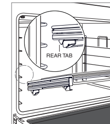
Install multifunction rack
